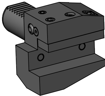
90DEG VDI30 STATIC TOOL OUTPUT: 20mm SQR SHANK COOLANT: EXTERNAL
